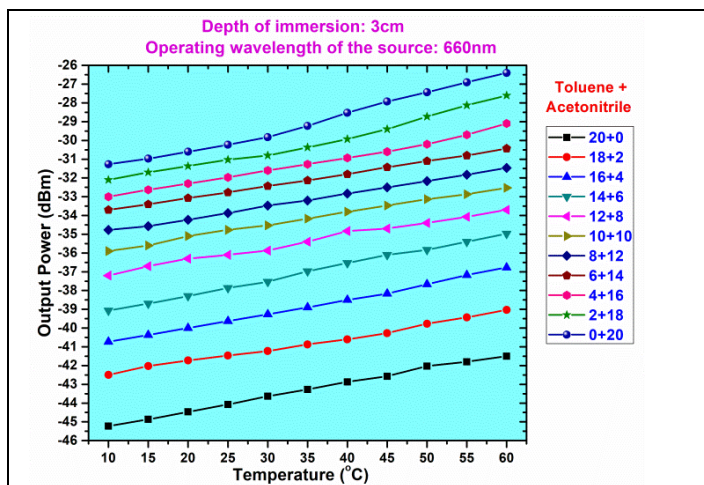
Fig.12: Relation between Temperature and Output power of Toluene + Acetonitrile mixtures at depth of immersion is 3cm
