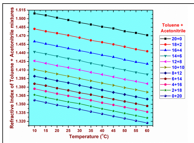
Fig.4: Relation between Temperature and Refractive index of Toluene + Acetonitrile mixtures.
