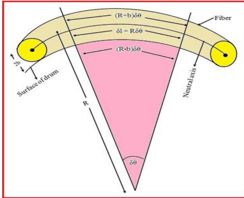
Fig.1: Surface strain produced by bending. Strain at outer surface (tension) = \frac{(R+b)\delta\theta - R\delta\theta}{R\delta\theta} = \frac{b}{R} = strain at inner surface (compression)
