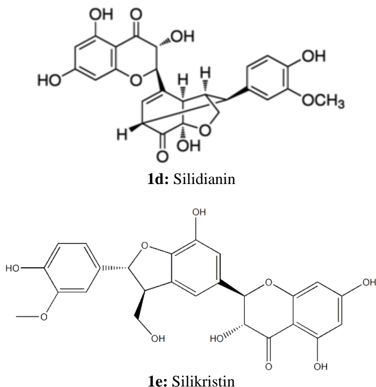
Fig.1.1 The chemical structure of some flavonolignans of Silymarin
